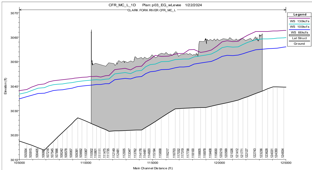
Figure 3-1. Modeled water surface elevations and berm profile.
