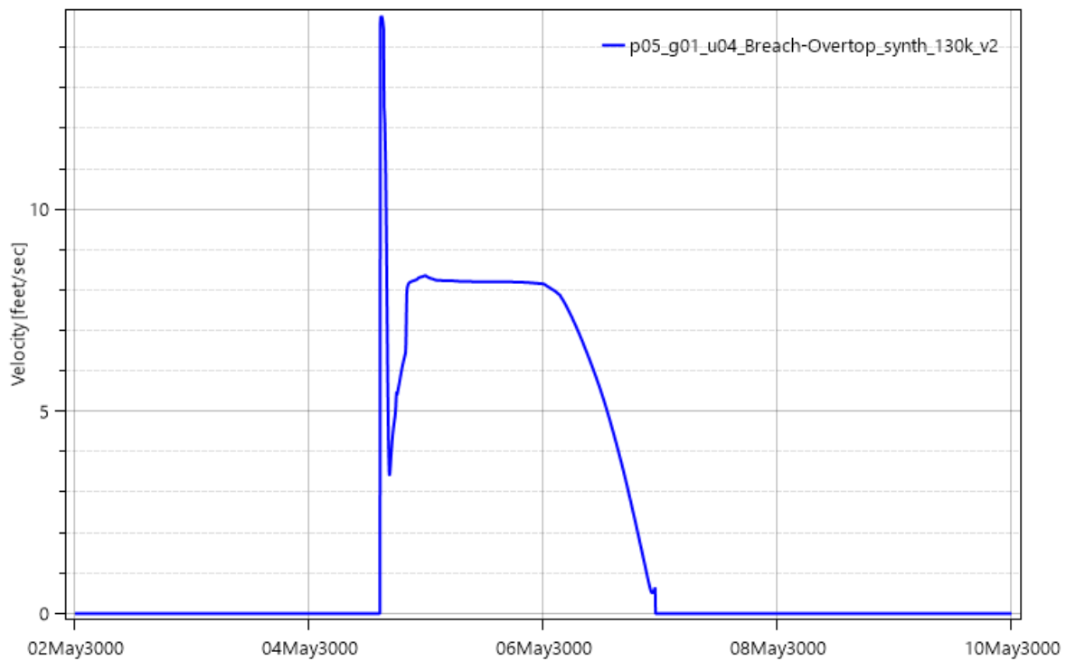
Figure 4-7. Plot of modeled velocity through the breach in the Scenario 3 overtopping failure.
