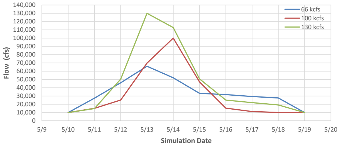
Figure 2-7. Synthetic flow hydrographs for historical and future flows.
