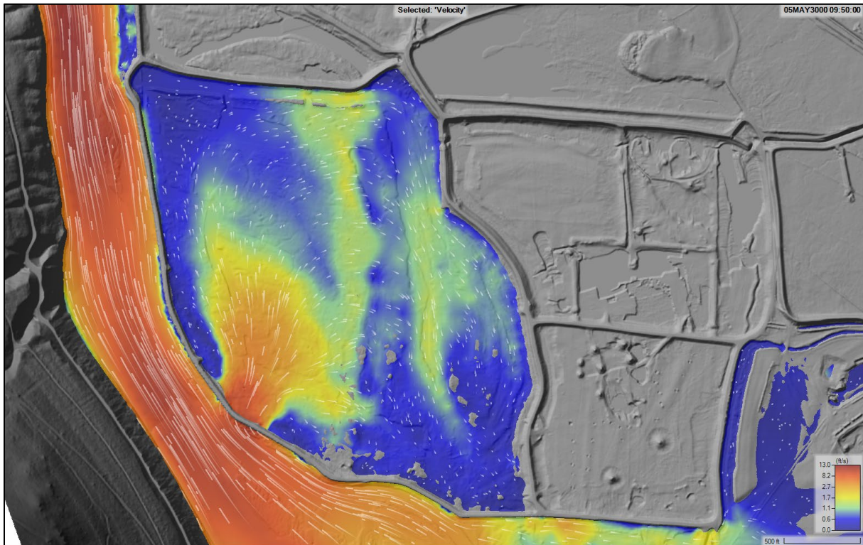
Figure 4-3. Plot of modeled velocities and particle traces at the peak of the Scenario 2 mass-wasting failure near the southeast end of Holding Pond 2.
