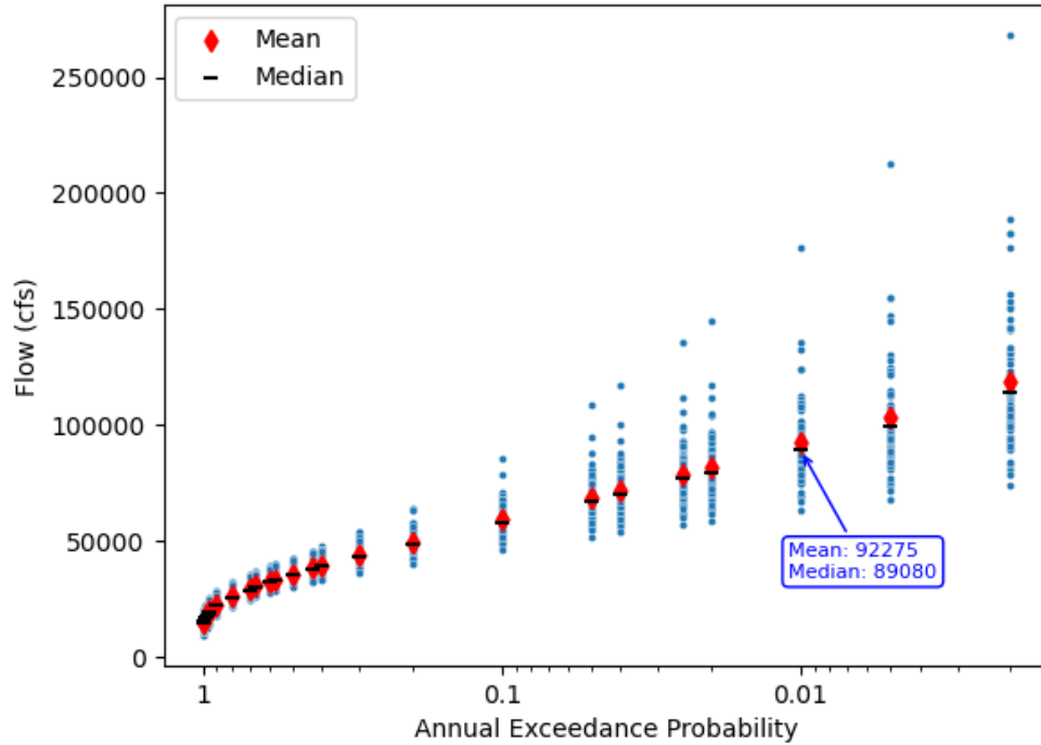
Figure A-1. Distribution of flood frequency quantiles for the CFR downstream of Missoula developed using modeled future flow data assuming a mid-range greenhouse gas scenario (RCP 4.5).
