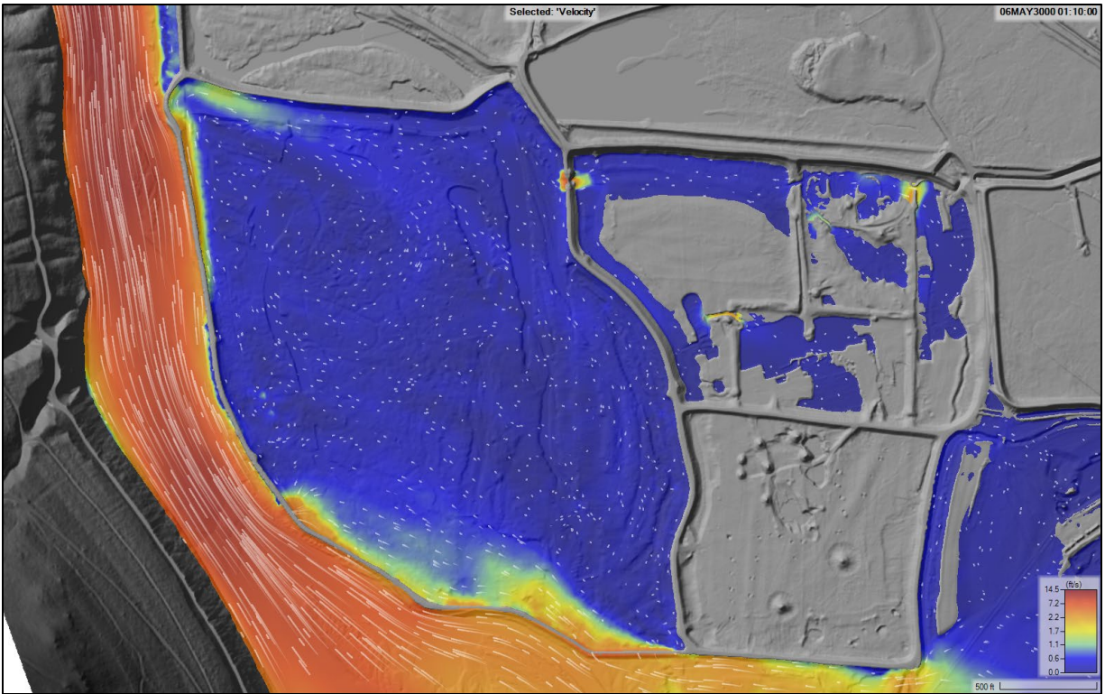
Figure 4-4. Plot of modeled velocities and particle traces for the Scenario 2 mass-wasting failure showing flow across the interior berm into Holding Pond 1.
