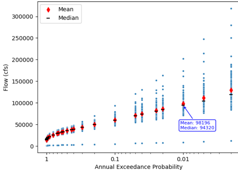
Figure A-2. Distribution of flood frequency quantiles for the CFR downstream of Missoula developed using modeled future flow data assuming a very high greenhouse gas scenario (RCP 8.5).
