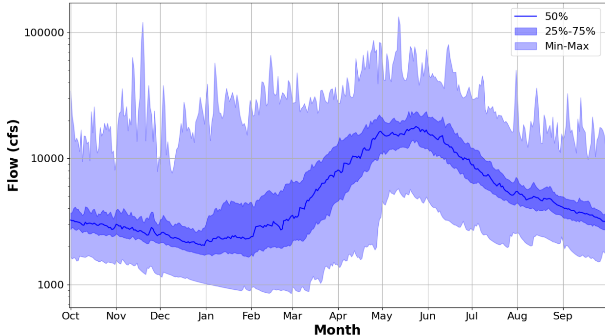
Figure 2-5. Summary hydrograph that exemplifies potential future flows under RCP 8.5.
