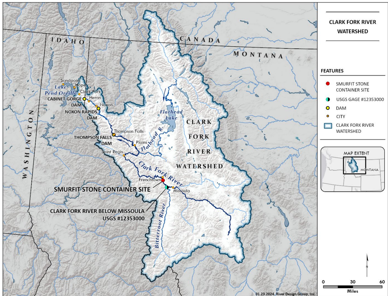
Figure 2-1. Study Reach watershed and gage map.
