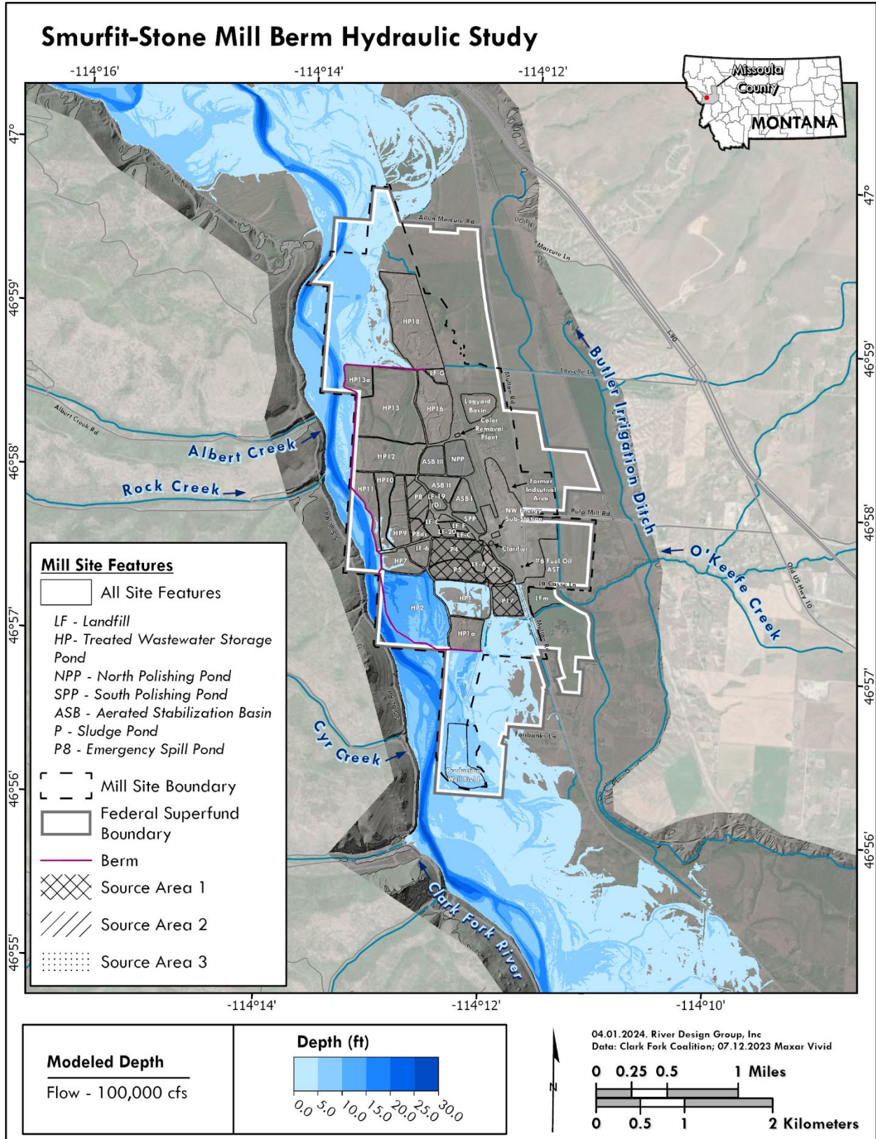
Figure B-3. Depth map for future 100-year flood event of ~100,000 cfs.
