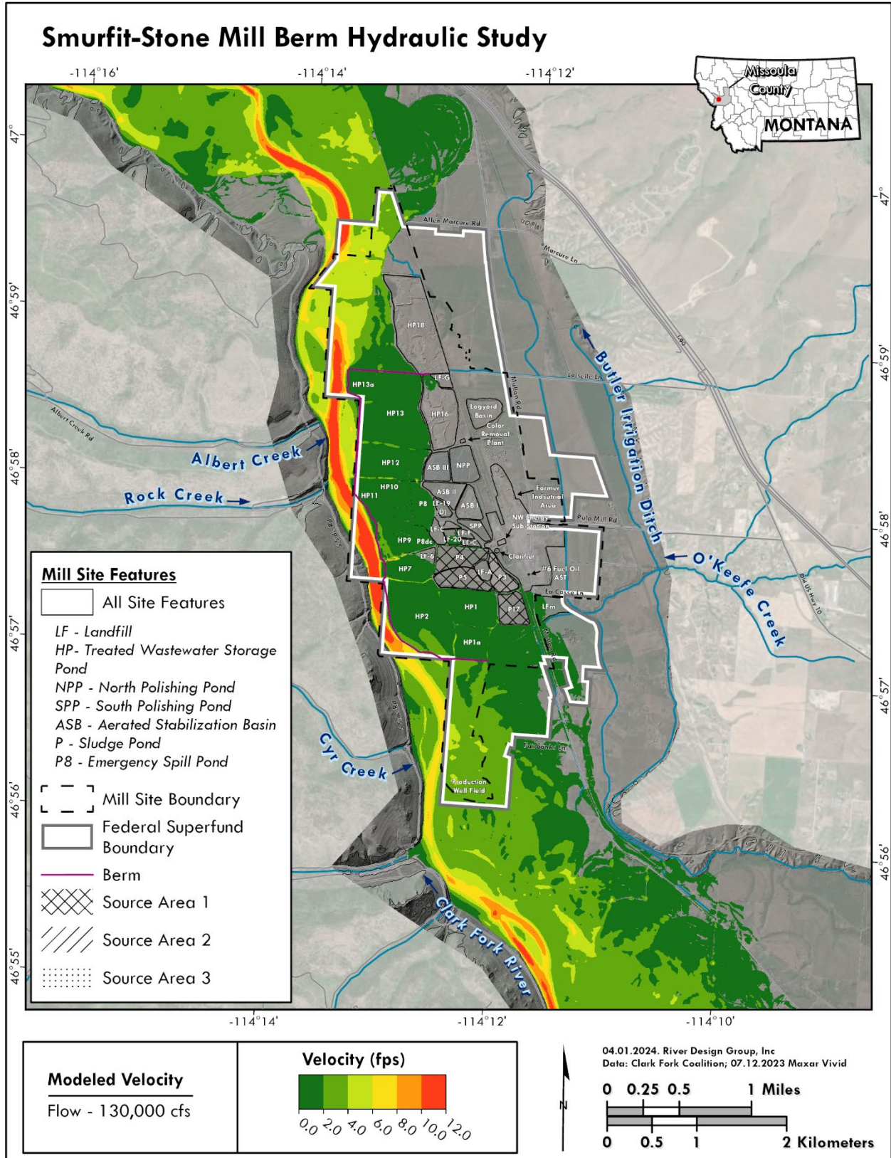
Figure B-6. Velocity map for future 500-year flood event of ~130,000 cfs.
