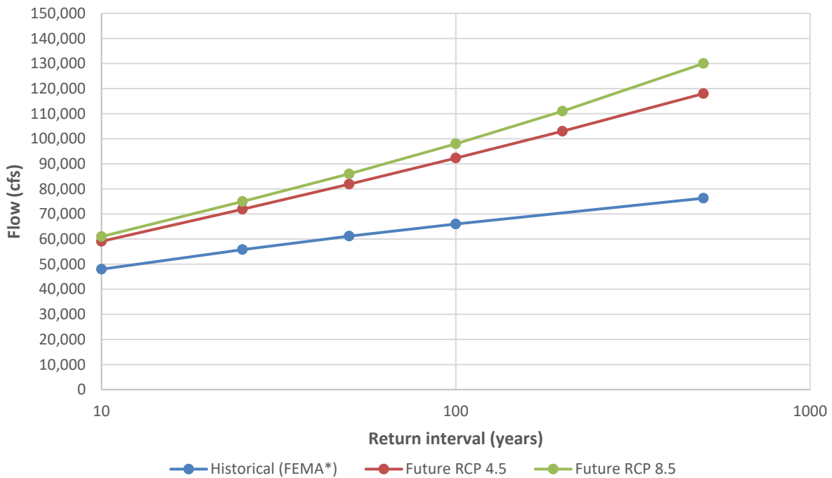
Figure 2-6. Comparison of flood quantiles for historical and future flows.
