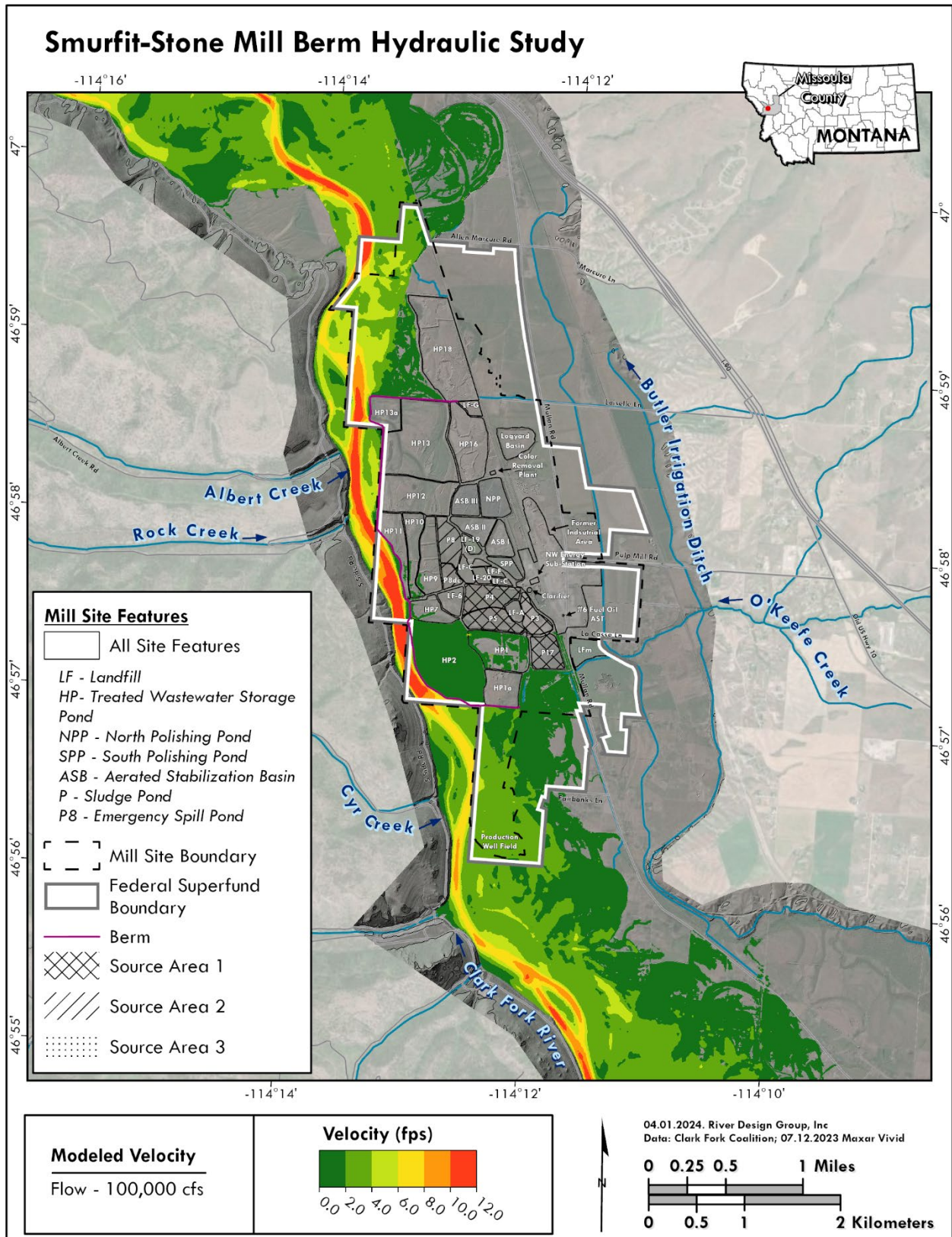
Figure B-4. Velocity map for future 100-year flood event of ~100,000 cfs.
