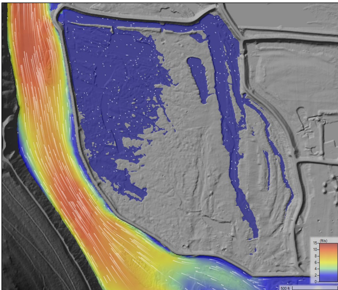
Figure 4-1. Plot of modeled velocities and particle traces for the Scenario 1 piping failure near the north end of Holding Pond 2.
