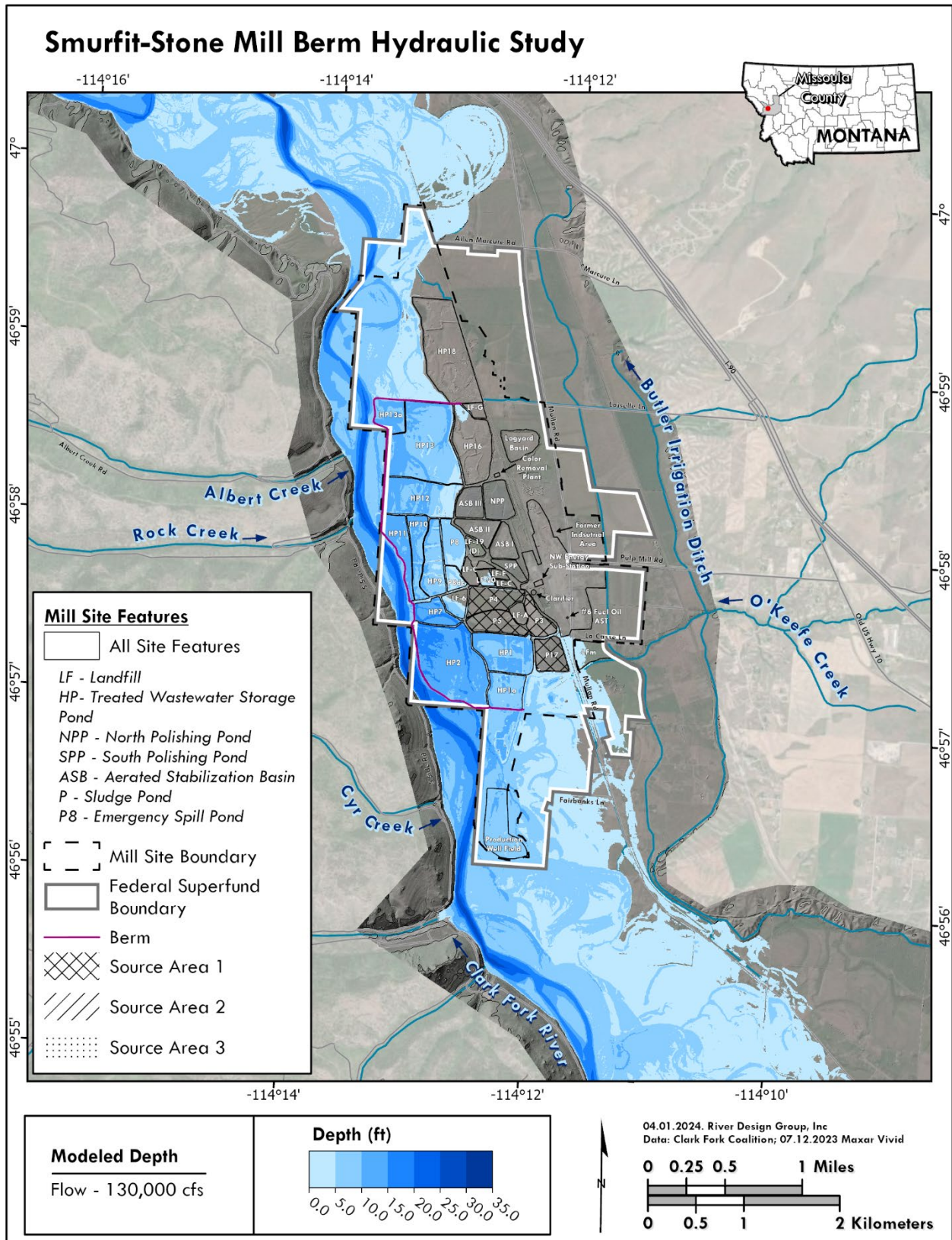
Figure B-5. Depth map for future 500-year flood event of ~130,000 cfs.
