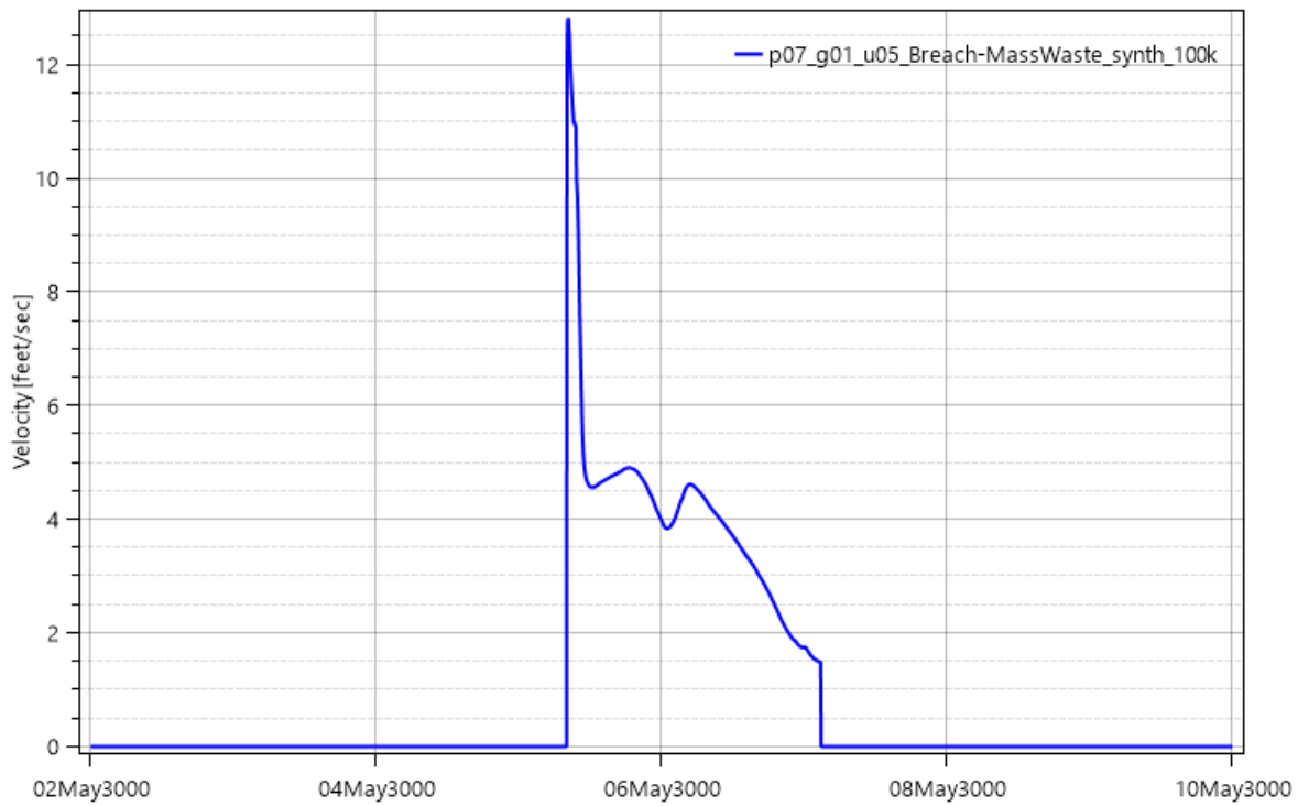
Figure 4-5. Plot of modeled velocity through the breach in the Scenario 2 mass-wasting failure.
