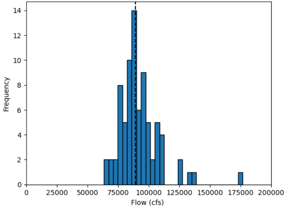
Figure A-3. Histogram of 1% annual chance (100-year) flows for the CFR downstream of Missoula developed using modeled future flow data assuming a mid-range greenhouse gas scenario (RCP 4.5).
