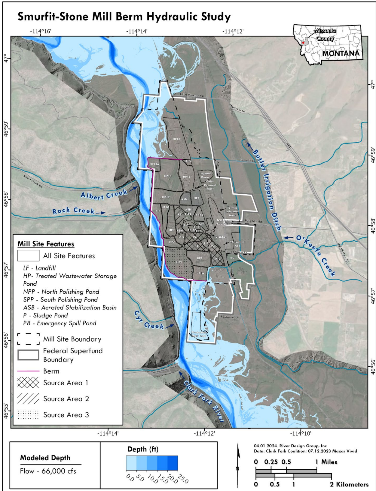
Figure B-1. Depth map for historical 100-year flood event of 66,000 cfs.
