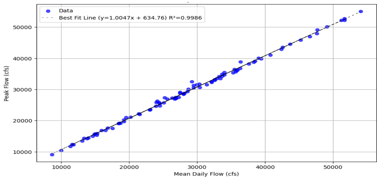
Figure 2-8. Comparison of daily flows with peak flows.
