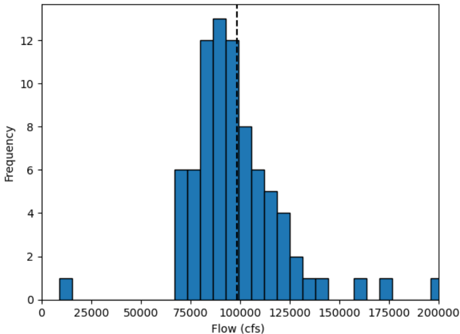
Figure A-4. Histogram of 1% annual chance (100-year) flows for the CFR downstream of Missoula developed using modeled future flow data assuming a very high greenhouse gas scenario (RCP 8.5).
