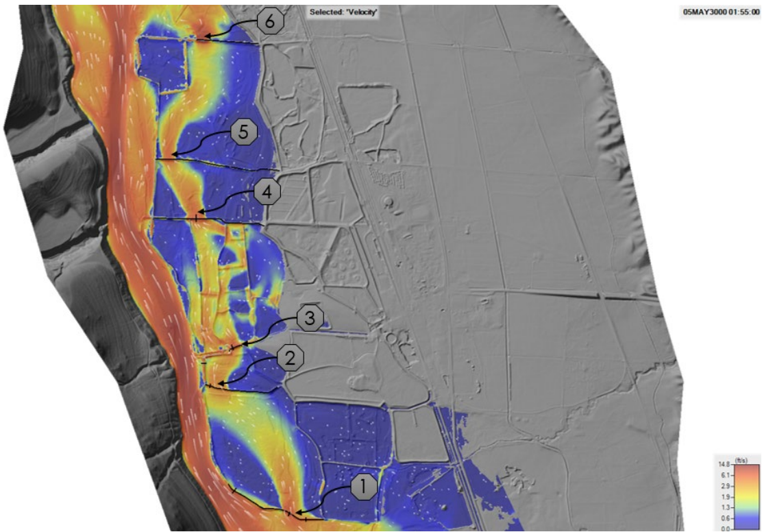
Figure 4-6. Plot of modeled velocities and particle traces at the peak of the Scenario 3 overtopping failure.
