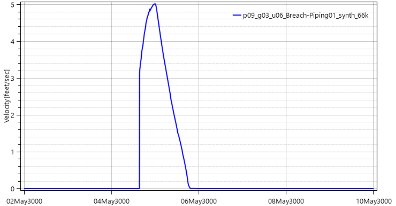
Figure 4-2. Plot of modeled velocities inside of berm at failure point for the Scenario 1 piping failure near the north end of Holding Pond 2.
