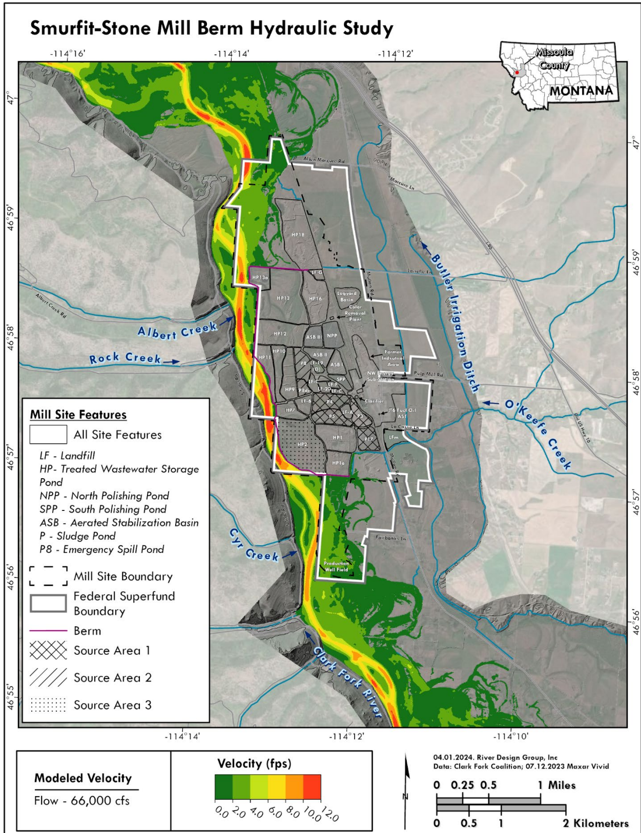
Figure B-2. Velocity map for historical 100-year flood event of 66,000 cfs.
