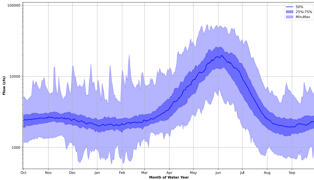
Figure 2-3. Summary hydrograph of CFR mean daily flows from 1927 through 2023.
