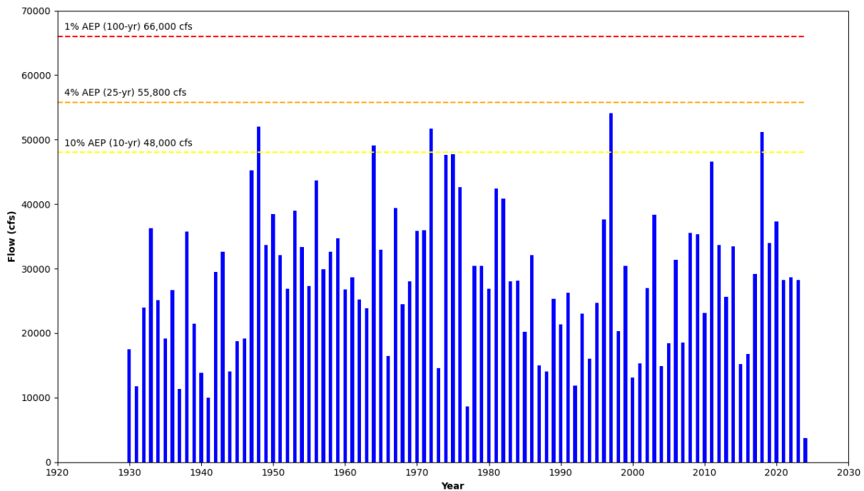
Figure 2-4. Summary hydrograph of CFR mean daily flows from 1927 through 2023.
